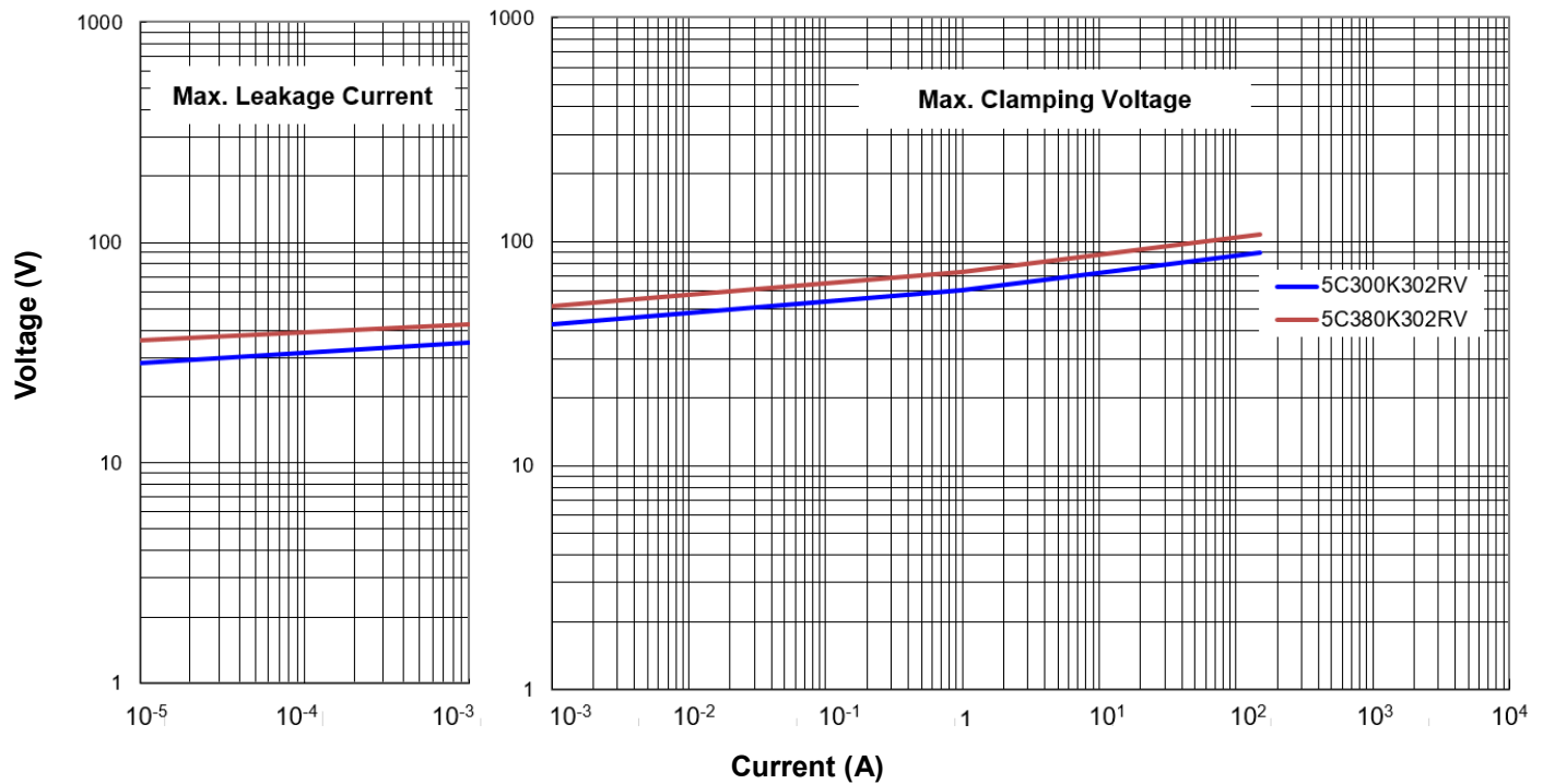
Max. Leakage Current and Max. Clamping Voltage Curves (TVM5C300K302RV, TVM5C380K302RV)
