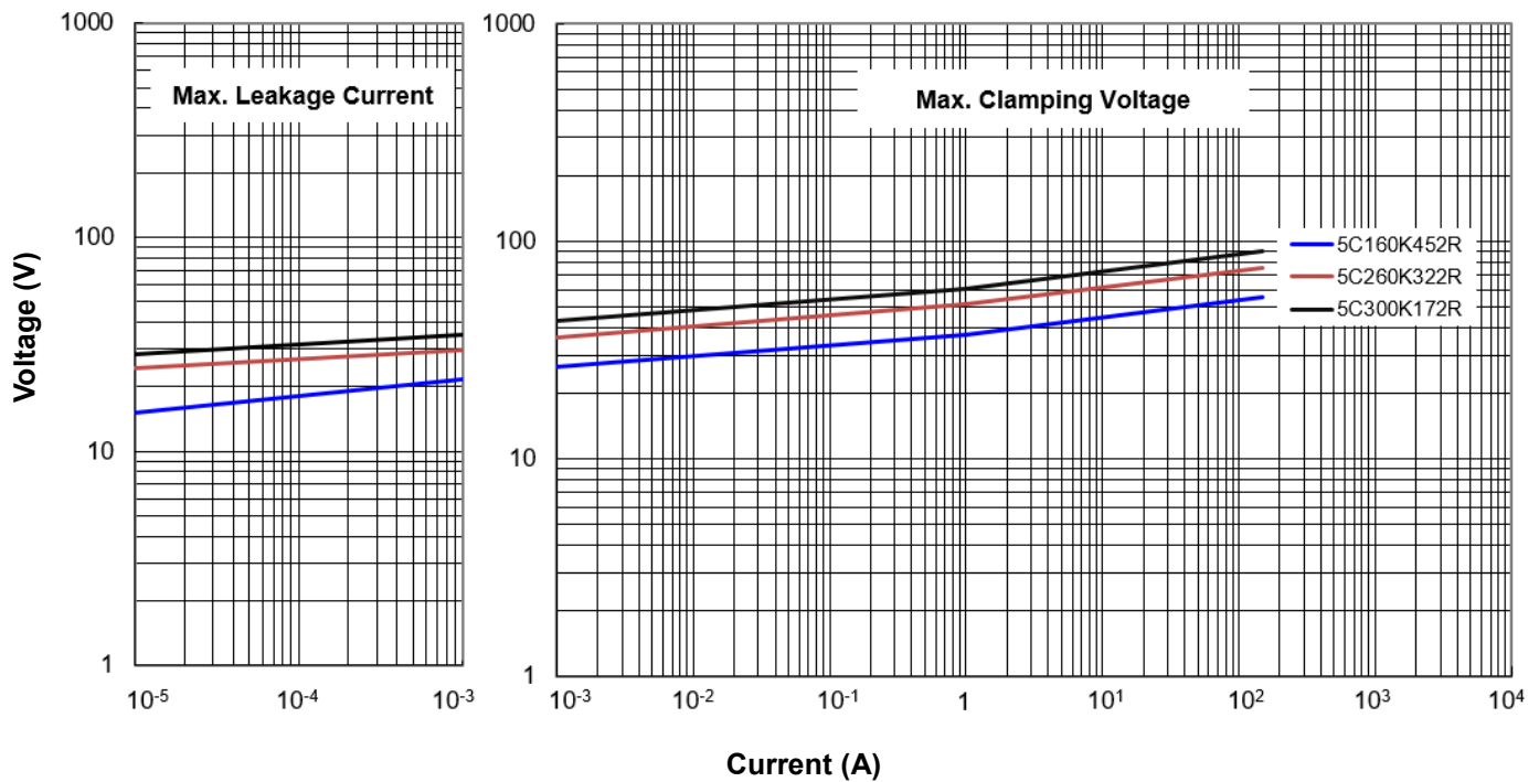
Max. Leakage Current and Max. Clamping Voltage Curves (TVM5C160K452R~TVM5C300K172R)
